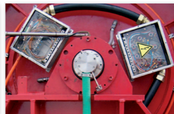
Slip ring installed on winch
